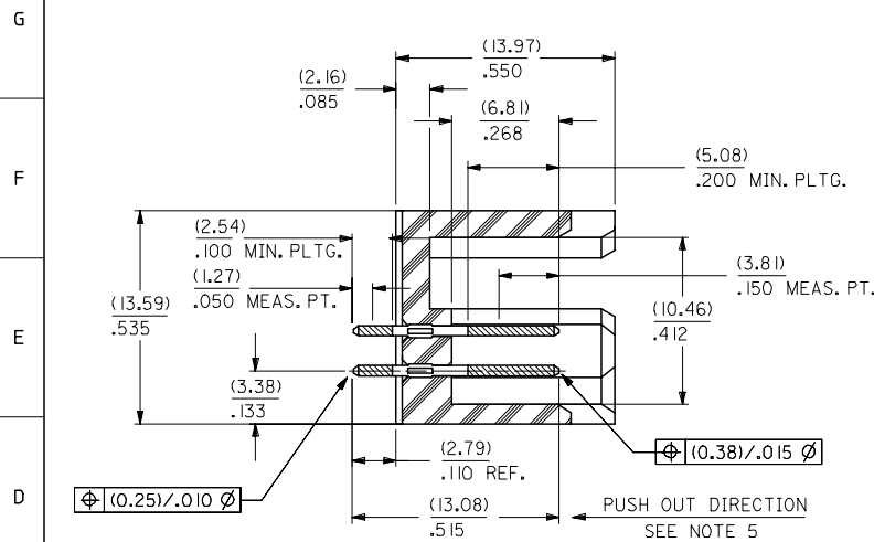
SECTION W-W
